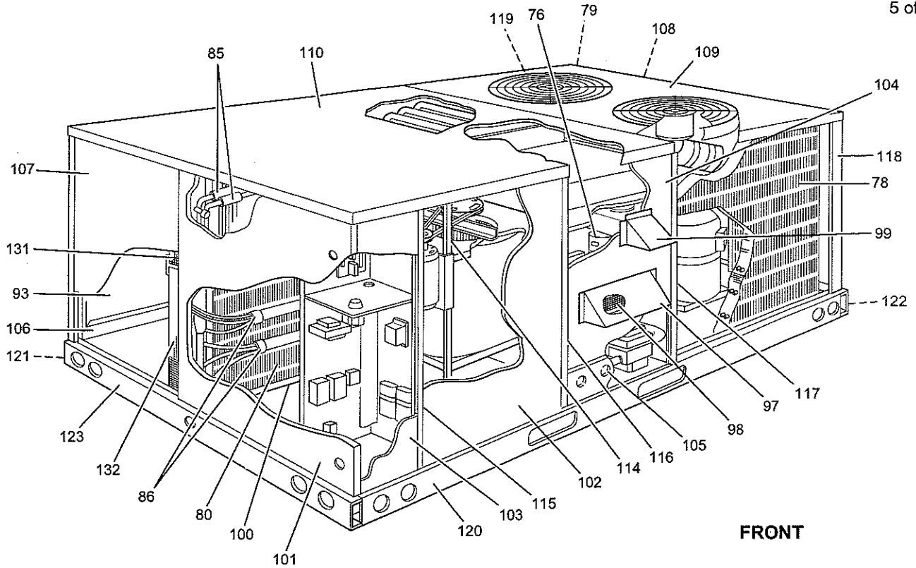
FIG. 4 – SINGLE PACKAGE GAS / ELECTRIC UNIT
