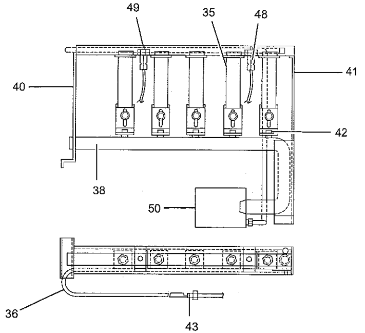
FIG. 3 - BURNER ASS'Y
